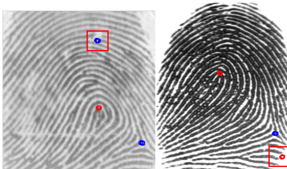
Fig. 9. Forged singular points detected using a conventional Poincare Index-based method and post-processing steps, in which the false points are marked with squares
