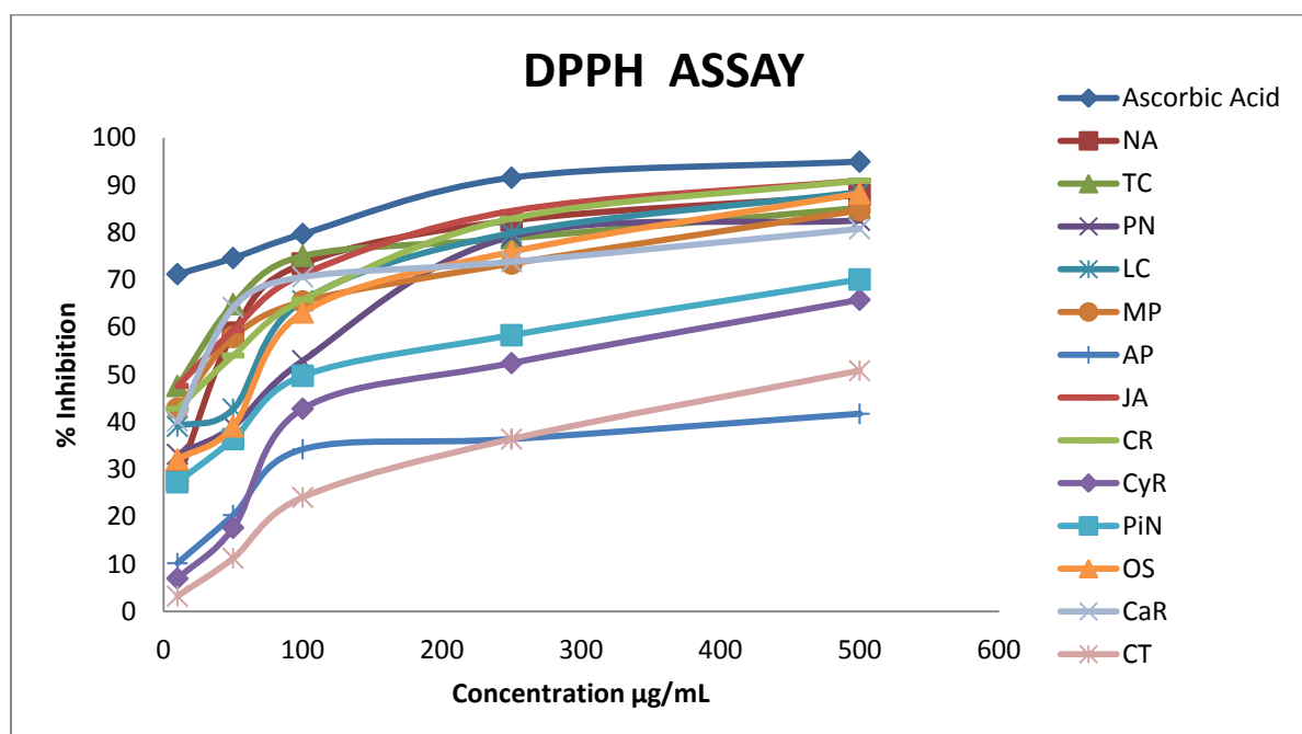
Fig. 1. DPPH free radical scavenging activity of methanolic plant extracts.
