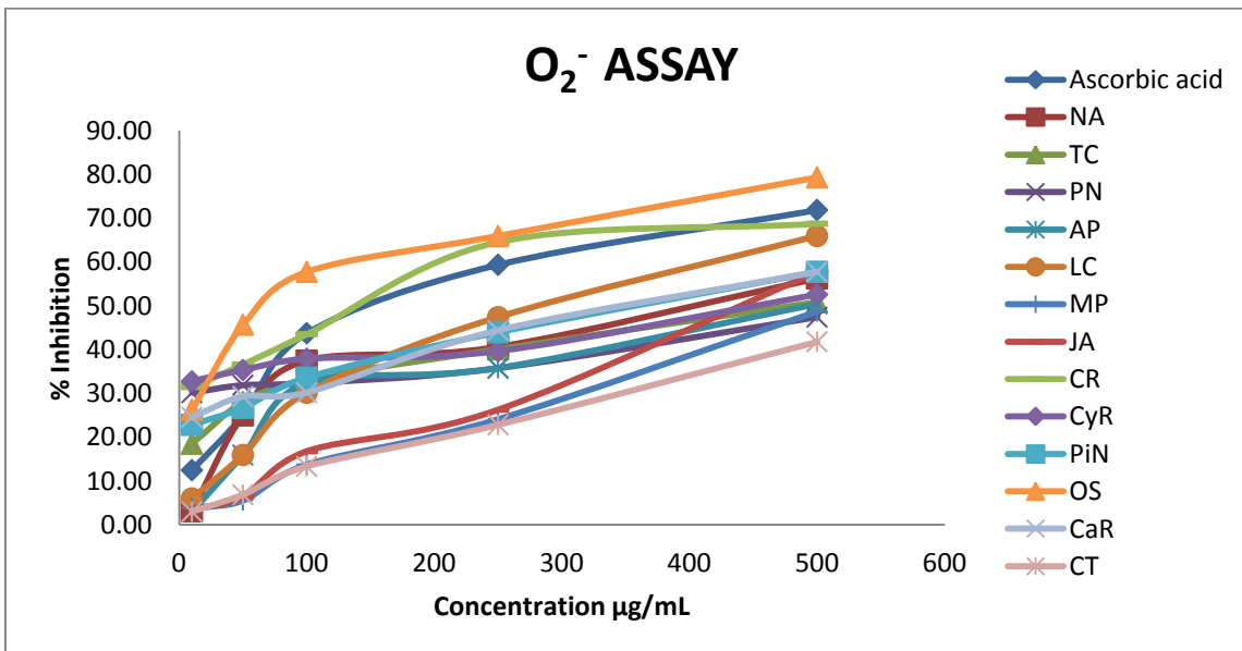
Fig. 3. Superoxide free radical scavenging activity of methanolic plant extracts
