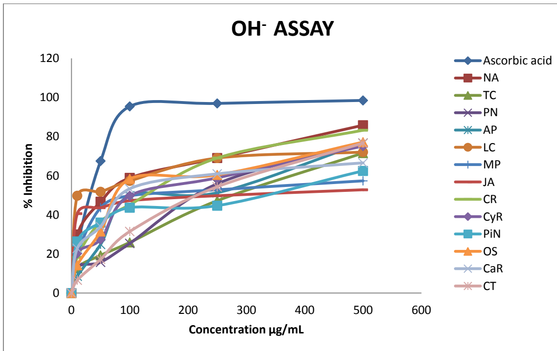
Fig. 2. Hydroxyl free radical scavenging activity of methanolic plant extracts.
