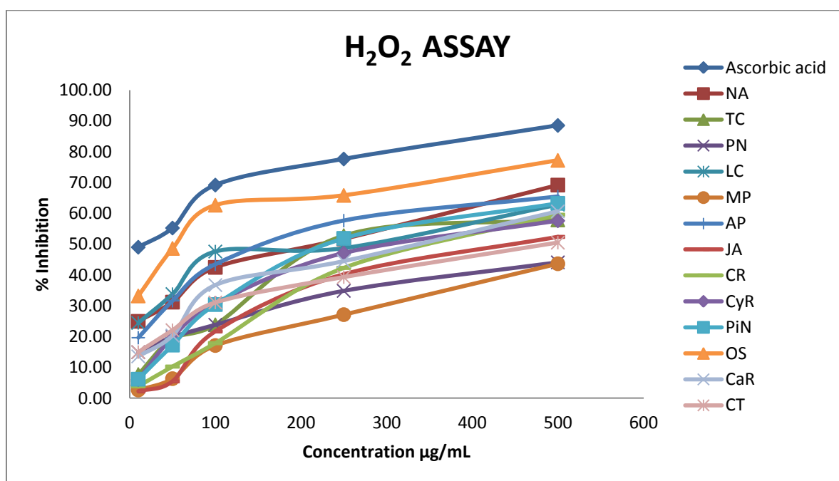
Fig. 4. Hydrogen peroxide (H 2 O 2 ) free radical scavenging activity of methanolic plant extracts
