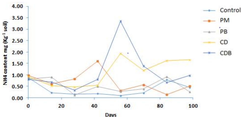
Fig. 5. NH 4 -N release in terrace soil as influenced by different organic materials during 14 weeks of incubation
