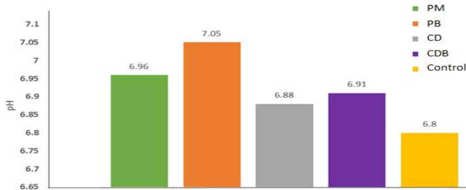
Fig. 2. Average pH values in terrace soil as influenced by different organic materials during 14 weeks of incubation
