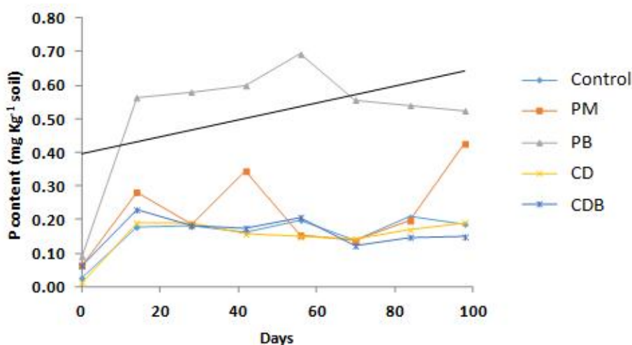
Fig. 6. P release in terrace soil as influenced by different organic materials during 14 weeks of incubation
