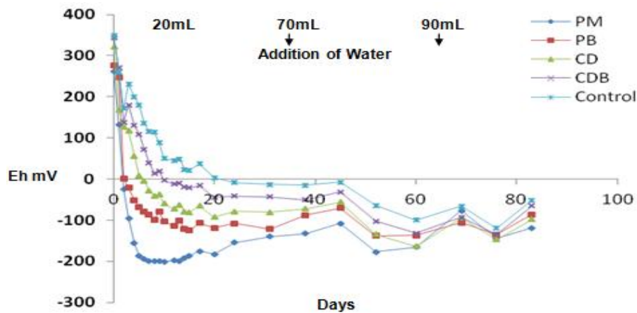
Fig. 3. Eh values in terrace organic materials during 14 weeks of incubation
