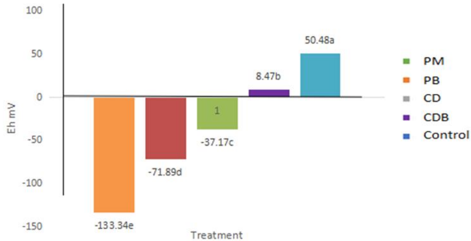
Fig. 4. Average Eh values in terrace soil as influenced by different organic materials during 14 weeks of incubation
