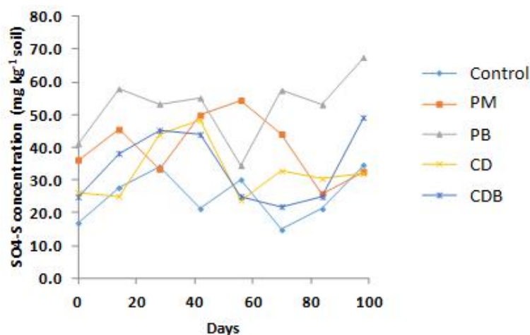
Fig. 7. SO 4 -S release in terrace soil as influenced by different organic materials during 14 weeks of incubation
