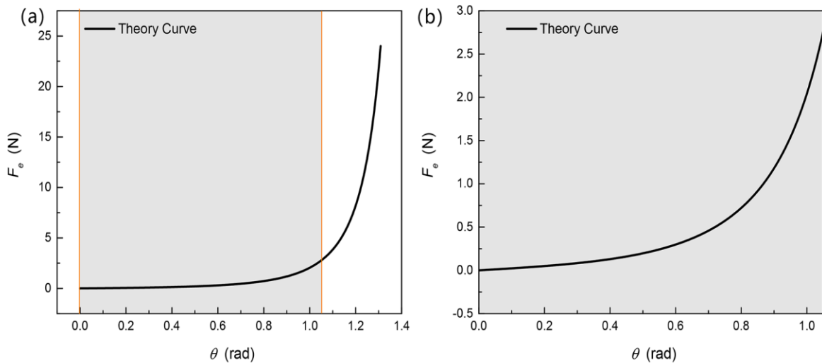
Fig. 2. (a) Theoretical curve of the horizontal external force versus the inclination angle. (b) The enlargement figure of the gray area in (a)
