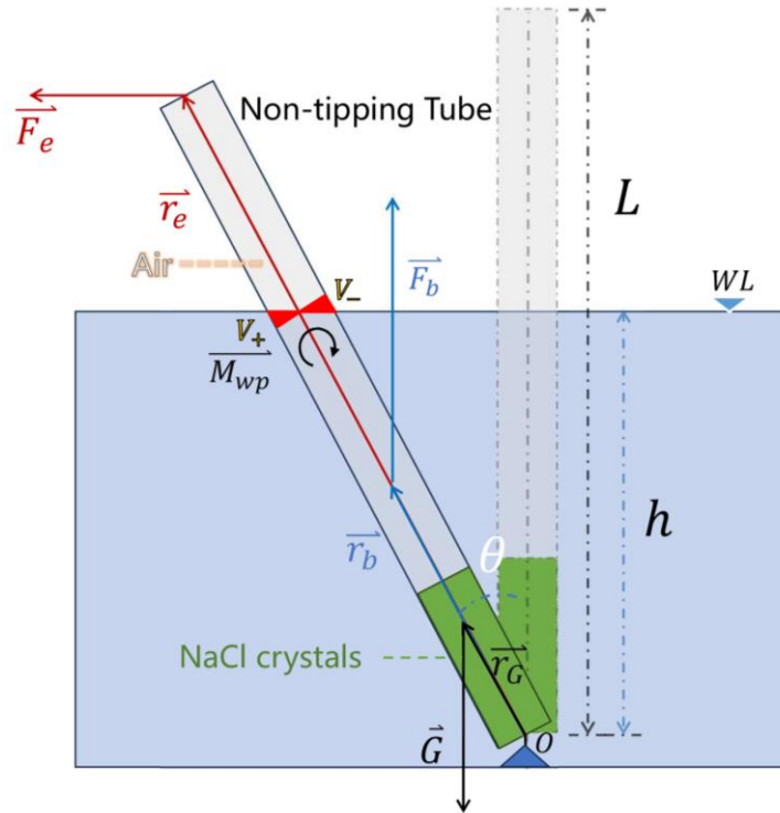
Fig. 1. Schematic diagram of the non-tipping tube device
