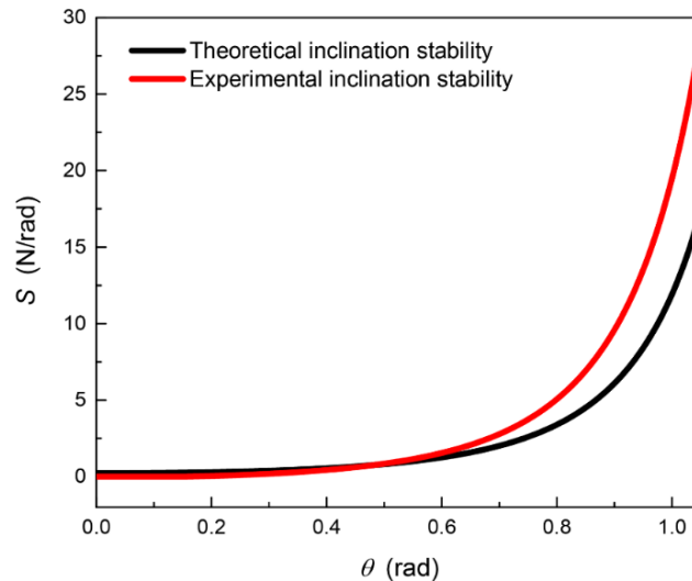
Fig. 6. Theoretical and experimental inclination stability curves
