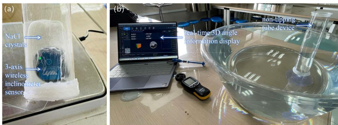
Fig. 4. (a) The interior diagram of the tube. (b)The computer displays real-time 3D angle information from the sensor
