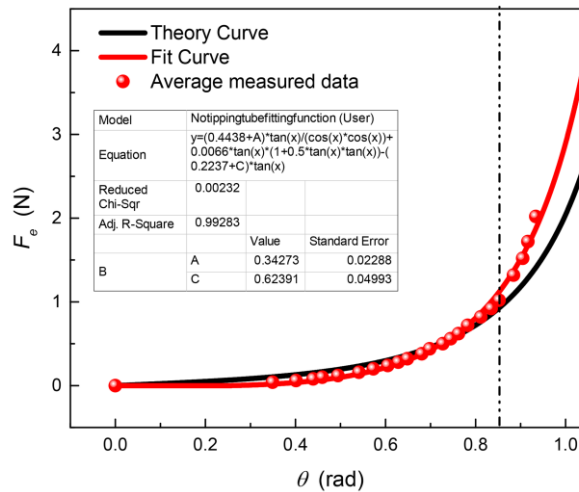
Fig. 5. The actual relationship between the horizontal external force and the tube inclination angle
