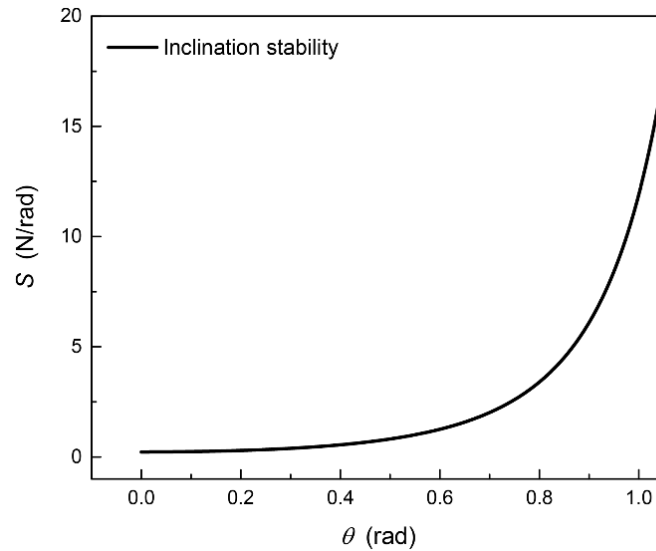
Fig. 3. Variation of theoretical stability with tube inclination angle
